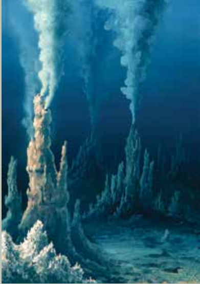
Hydrothermal vents
