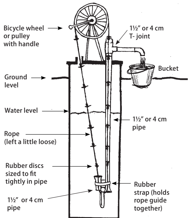
The rope pump is made from low cost, durable parts.
