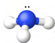
Figure 18.29 The structure of ammonia is shown with a central nitrogen atom and three hydrogen atoms.
