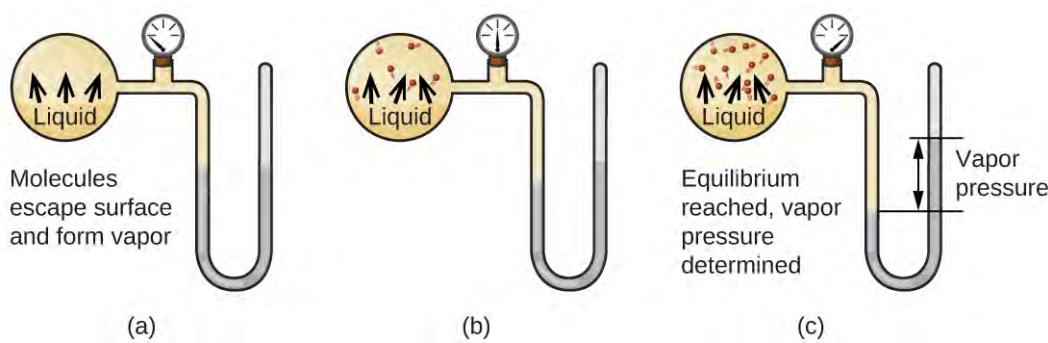
Figure 10.22 In a closed container, dynamic equilibrium is reached when (a) the rate of molecules escaping from the liquid to become the gas (b) increases and eventually (c) equals the rate of gas molecules entering the liquid. When this equilibrium is reached, the vapor pressure of the gas is constant, although the vaporization and condensation processes continue.
