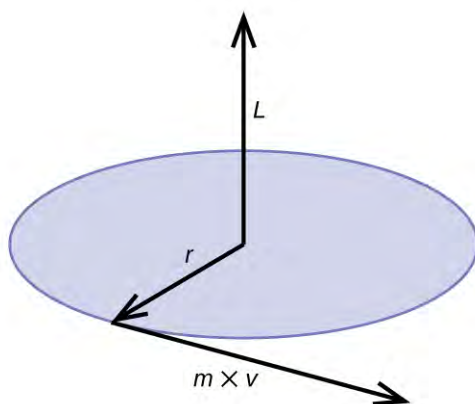
Figure 6.18 The diagram shows angular momentum for a circular motion.
