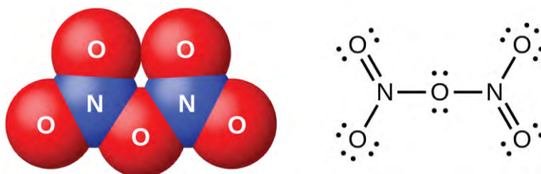
Figure 18.38 This image shows the molecular structure and one resonance structure of a molecule of dinitrogen pentaoxide, \text{N}_2\text{O}_5 .
