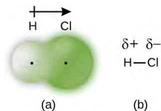
Figure 7.5 (a) The distribution of electron density in the HCl molecule is uneven. The electron density is greater around the chlorine nucleus. The small, black dots indicate the location of the hydrogen and chlorine nuclei in the molecule. (b) Symbols \delta^+ and \delta^- indicate the polarity of the H–Cl bond.
