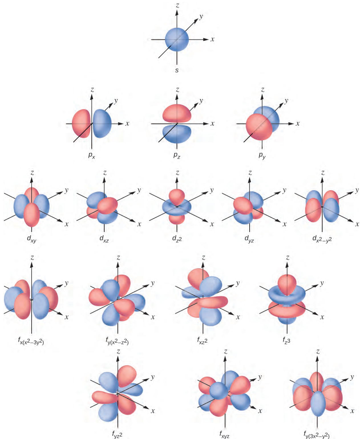
Figure 6.22 Shapes of s , p , d , and f orbitals.
