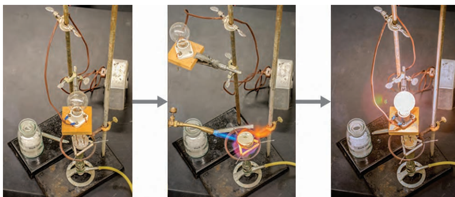
Figure 2.30 Sodium chloride melts at 801\text{ }^\circ\text{C} and conducts electricity when molten. (credit: modification of work by Mark Blaser and Matt Evans)
