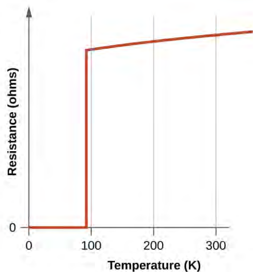
Figure 19.10 The resistance of the high-temperature superconductor \text{YBa}_2\text{Cu}_3\text{O}_7 varies with temperature. Note how the resistance falls to zero below 92 K, when the substance becomes superconducting.
