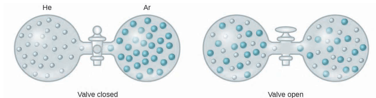
Figure 11.3 Samples of helium and argon spontaneously mix to give a solution in which the disorder of the atoms of the two gases is increased.
