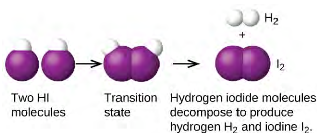
Figure 12.19 The probable mechanism for the dissociation of two HI molecules to produce one molecule of \text{H}_2 and one molecule of \text{I}_2 .
