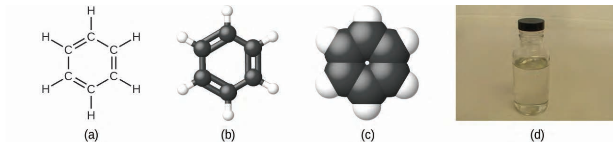
Figure 2.20 Benzene, C_6H_6 , is produced during oil refining and has many industrial uses. A benzene molecule can be represented as (a) a structural formula, (b) a ball-and-stick model, and (c) a space-filling model. (d) Benzene is a clear liquid. (credit d: modification of work by Sahar Atwa)
