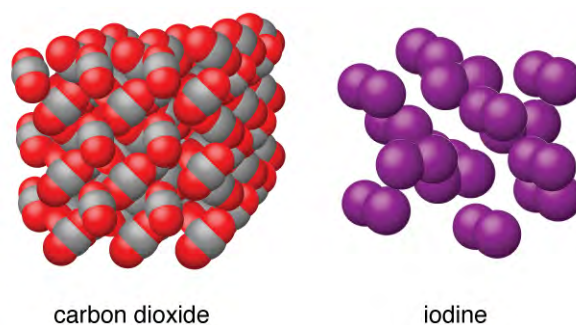
Figure 10.42 Carbon dioxide ( \text{CO}_2 ) consists of small, nonpolar molecules and forms a molecular solid with a melting point of -78\text{ }^\circ\text{C} . Iodine ( \text{I}_2 ) consists of larger, nonpolar molecules and forms a molecular solid that melts at 114\text{ }^\circ\text{C} .
