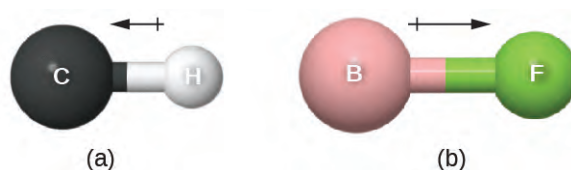
Figure 7.26 (a) There is a small difference in electronegativity between C and H, represented as a short vector. (b) The electronegativity difference between B and F is much larger, so the vector representing the bond moment is much longer.
