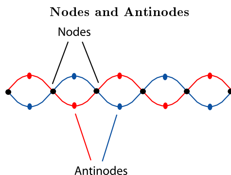
Figure 3.8: As a standing wave waves back and forth (from the red to the blue position), there are some spots called nodes that do not move at all; basically there is no change, no waving up-and-down (or back-and-forth), at these spots. The spots at the biggest part of the wave - where there is the most change during each wave - are called antinodes .
