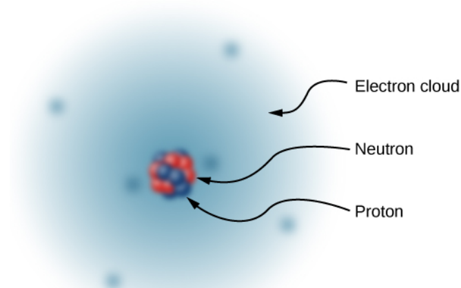
Figure 5.8 The nucleus of a carbon atom is composed of six protons and six neutrons. As in hydrogen, the surrounding six electrons do not have definite locations and so can be considered to be a sort of cloud surrounding the nucleus.
