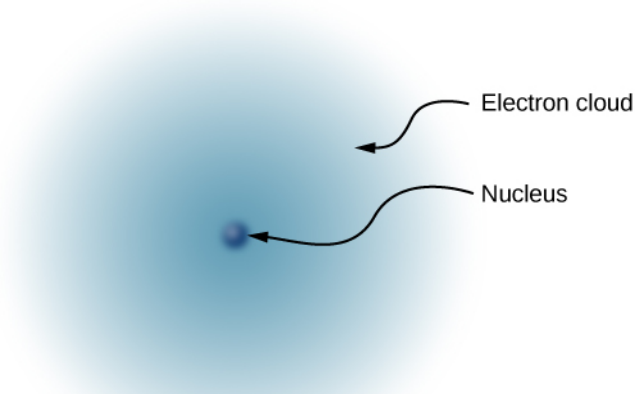
Figure 5.7 This simplified model of a hydrogen atom shows a positively charged nucleus (consisting, in the case of hydrogen, of a single proton), surrounded by an electron “cloud.” The charge of the electron cloud is equal (and opposite in sign) to the charge of the nucleus, but the electron does not have a definite location in space; hence, its representation here is as a cloud. Normal macroscopic amounts of matter contain immense numbers of atoms and molecules, and, hence, even greater numbers of individual negative and positive charges.
