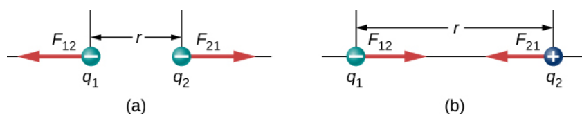
Figure 5.14 The electrostatic force \vec{F} between point charges q_1 and q_2 separated by a distance r is given by Coulomb's law. Note that Newton's third law (every force exerted creates an equal and opposite force) applies as usual—the force on q_1 is equal in magnitude and opposite in direction to the force it exerts on q_2 . (a) Like charges; (b) unlike charges.
