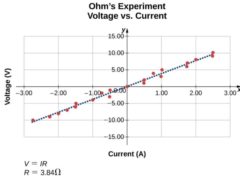
Figure 9.20 A resistor is placed in a circuit with a battery. The voltage applied varies from -10.00\ \text{V} to +10.00\ \text{V} , increased by 1.00\text{-V} increments. A plot shows values of the voltage versus the current typical of what a casual experimenter might find.
