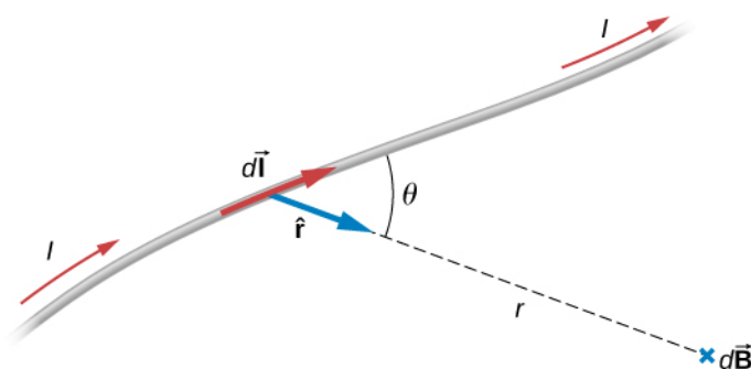
Figure 12.2 A current element I d\vec{\mathbf{I}} produces a magnetic field at point P given by the Biot-Savart law.
