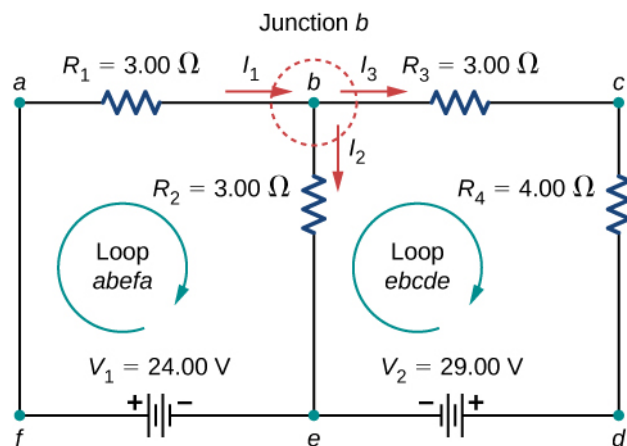
Figure 10.28 Choose the loops in the circuit.
